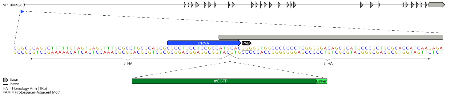
Figure 1: Top: POLR2A locus; Bottom: Zoom in on mEGFP insertion site at POLR2A N-terminal exon.
