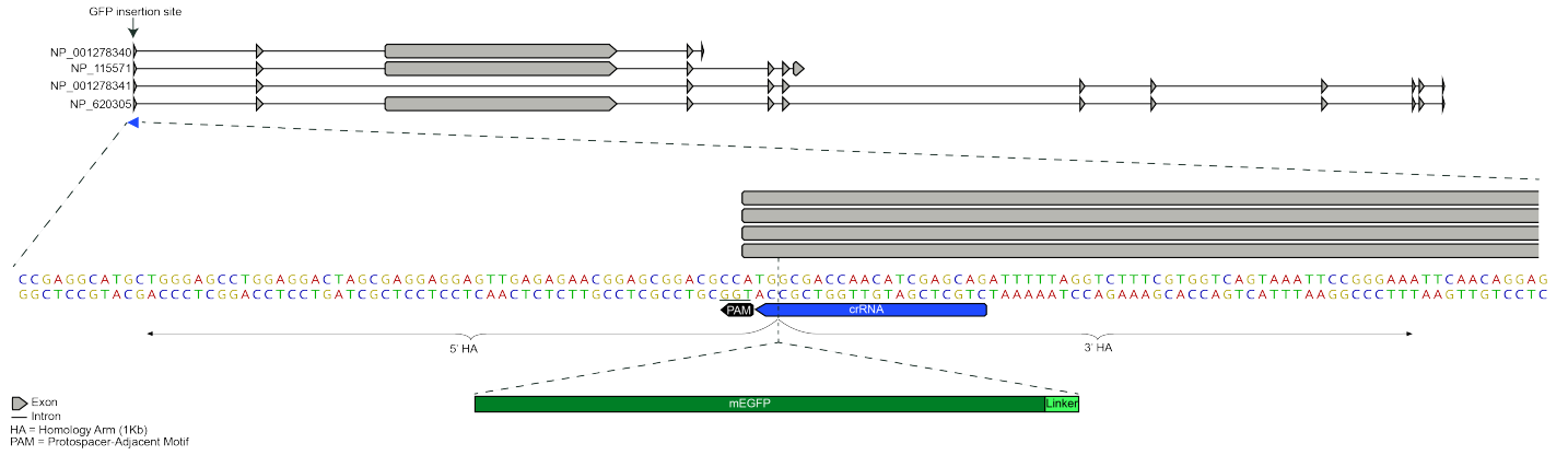
Figure 1: Top: SON locus showing 4 SON isoforms; Bottom: Zoom in on mEGFP insertion site at SON N-terminal exon
