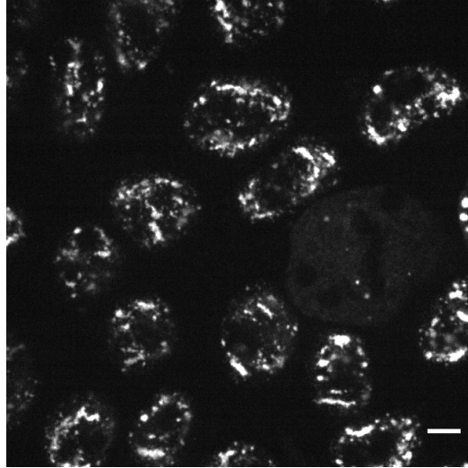
Figure 3: Single, mid-level plane of cells in a live hiPS cell colony expressing mEGFP-tagged SON. Cells were imaged in 3D on a spinning-disk confocal microscope. Scale bar, 5 \mu\text{m} .
