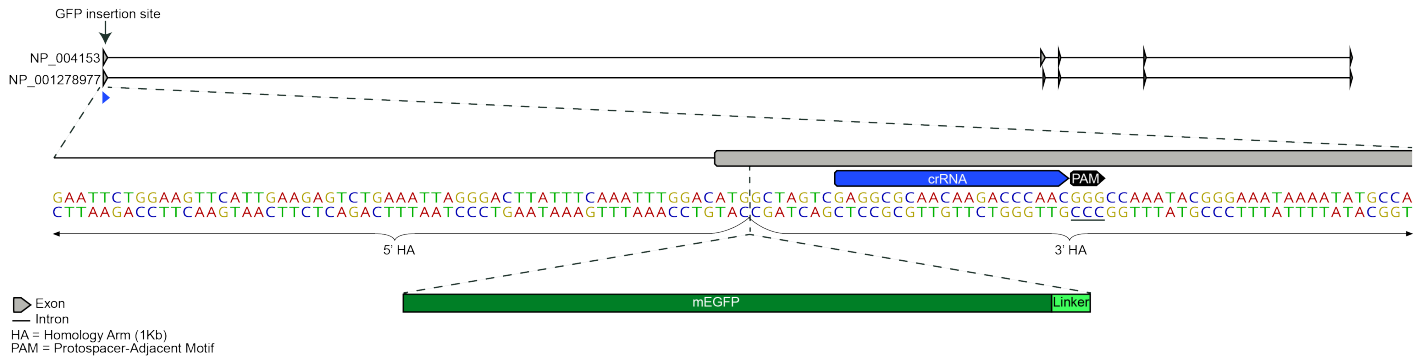
Figure 1: Top: RAB5A locus showing 2 RAB5A isoforms; Bottom: Zoom in on mEGFP insertion site at RAB5A N-terminal exon
